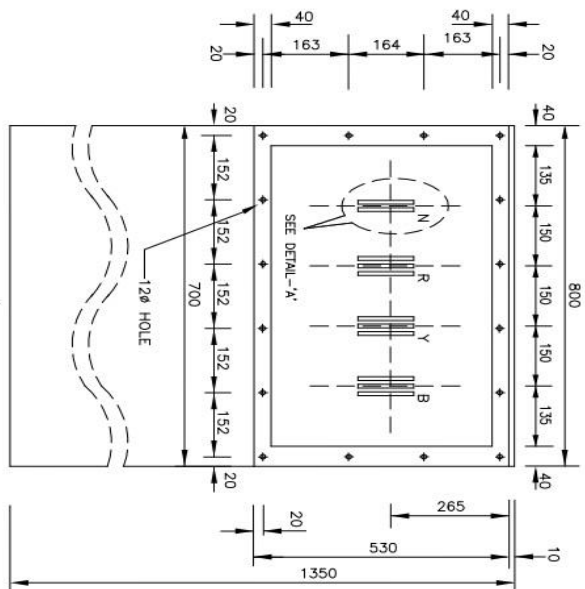
TOP VIEW FRONT
